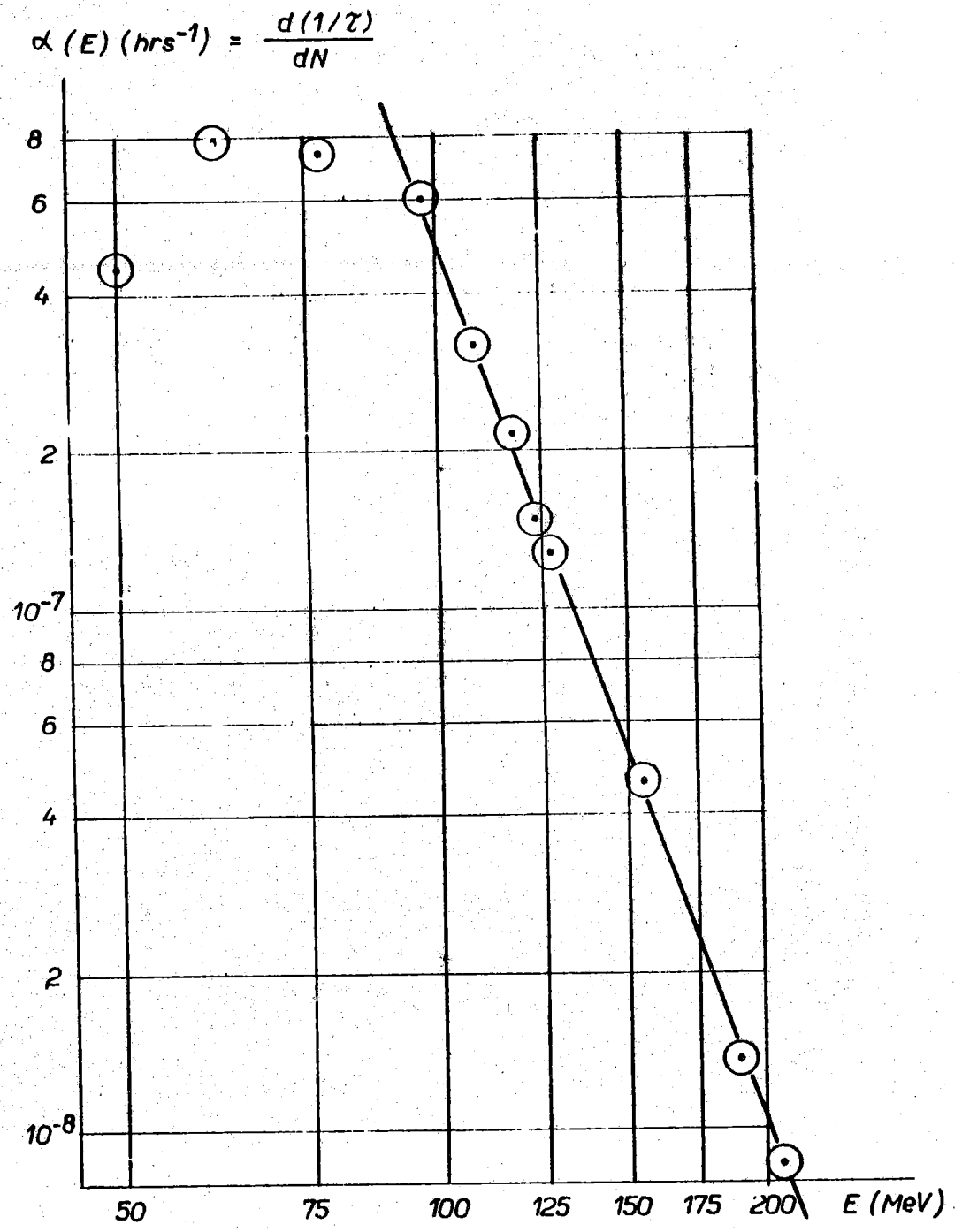
FIG. 2 - Plot of the rate \alpha(E) , as defined in eq. (1) of the text, versus the energy of electrons in a beam.
